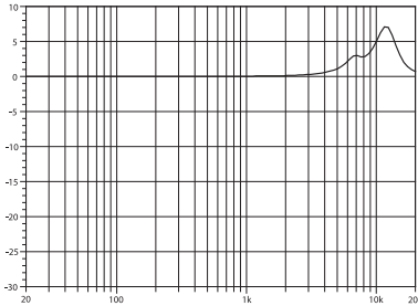
Fig. 4: Frequency response correction of HFC circuit
