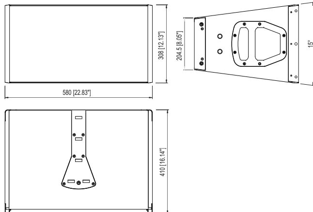
Fig. 9: Q1 cabinet dimensions in mm [inch]
